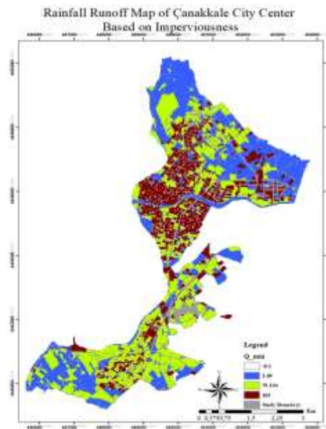
Figure 6. Rainfall Runoff Based on Imperviousness
